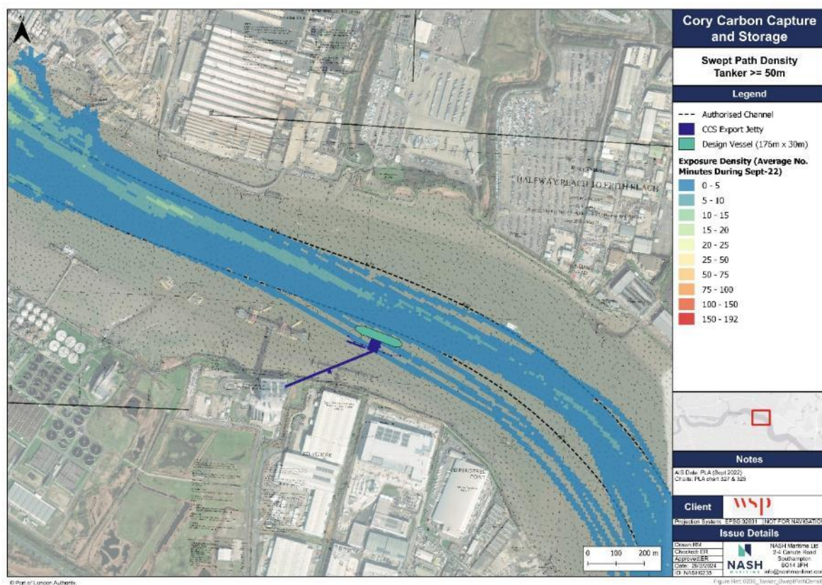
Figure 38: Tanker Swept Path Density Plot
