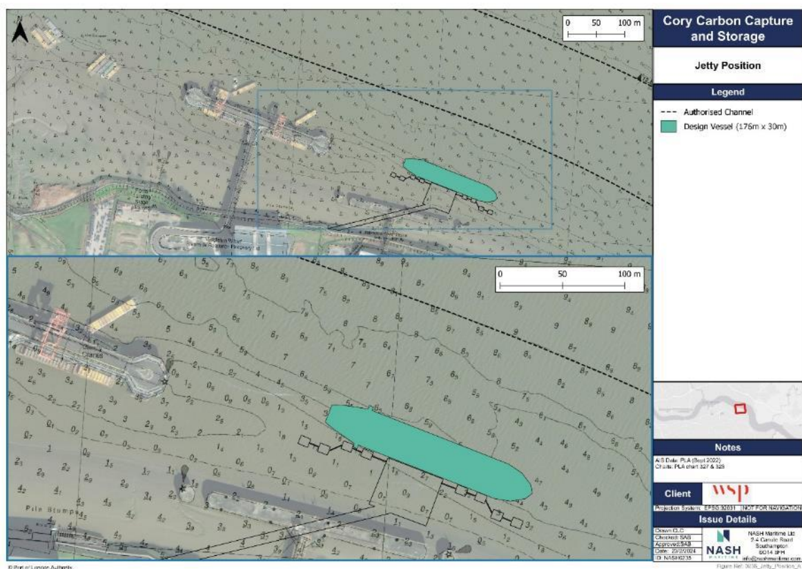
Figure 4: Jetty Option B
